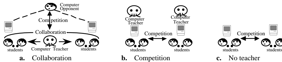
Fig. 2. Learning Models
